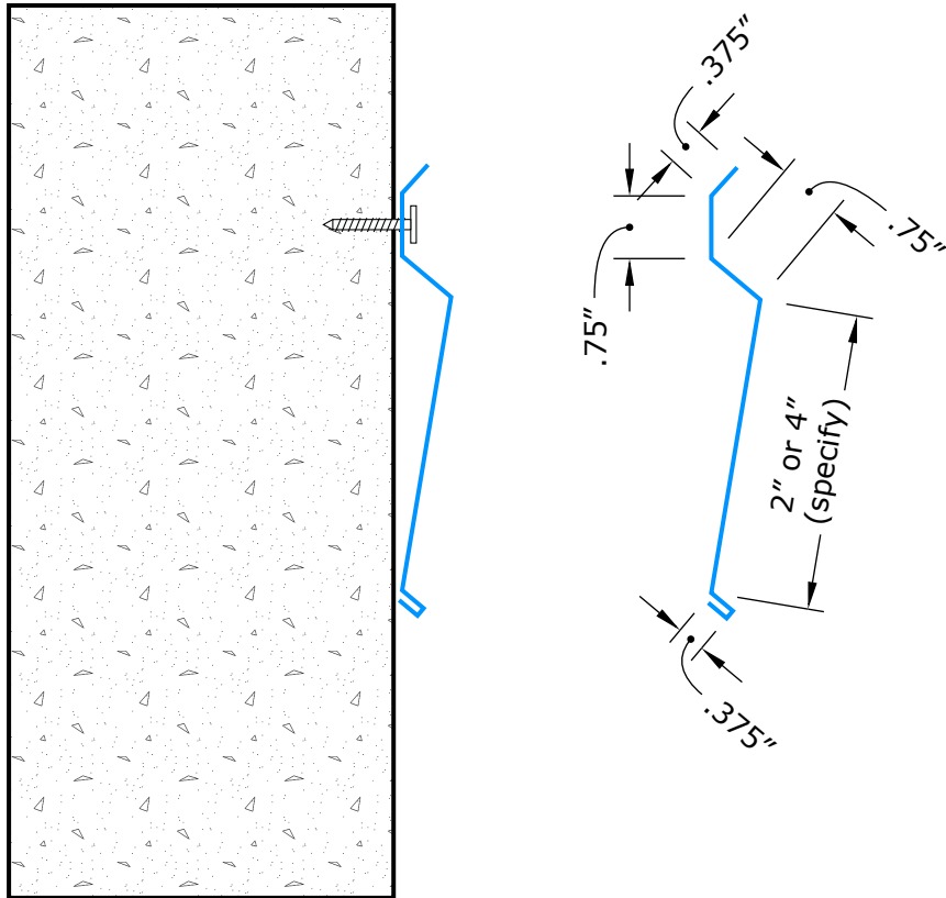
SMR1 "Flush Mount"
